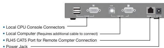
Receiver Unit
