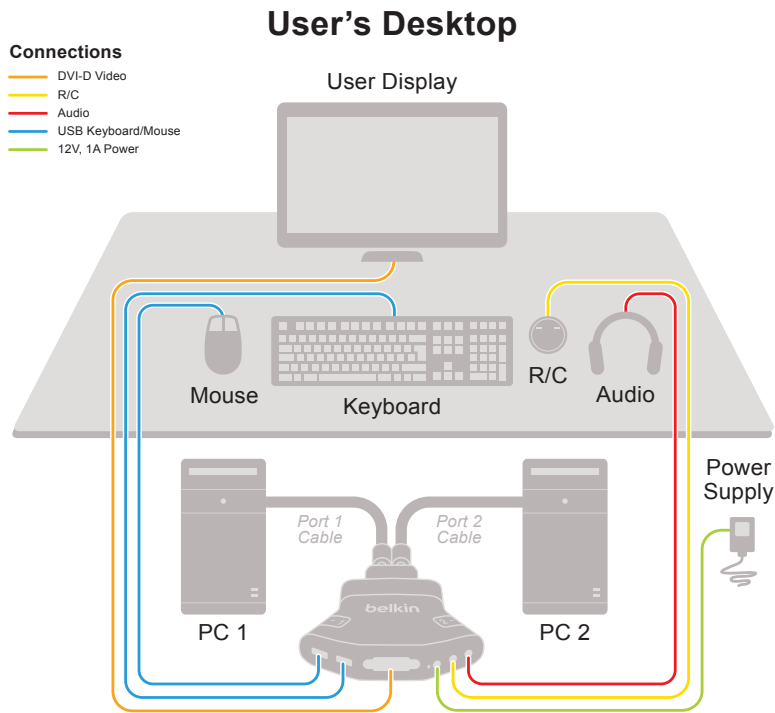
F1DN102F-3 Belkin Advanced Secure 2-Port Flip KVM
